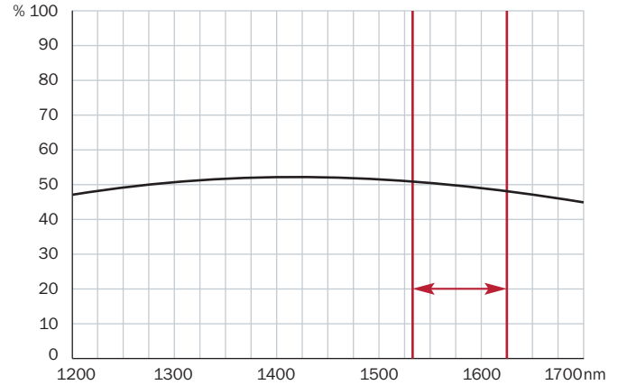
Wavelength dependence of Coupling Ratio of symmetrical C- & L-Band Coupler
